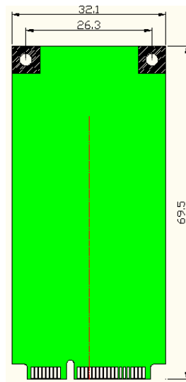
Photo2: Custom size (69.5x32.1mm)
