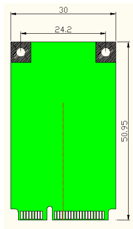
Photo1: Full size (50.95x30mm)
